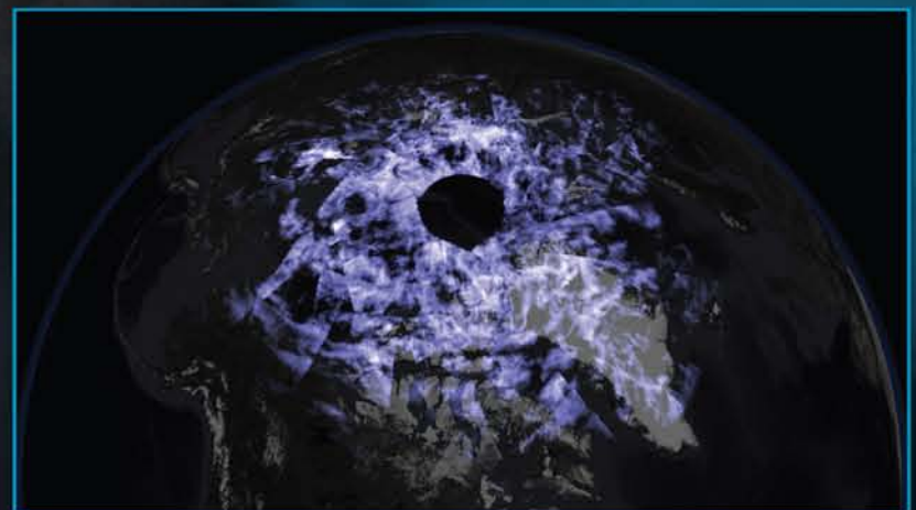
SOFIE Northern and Southern Season Ice Measurement Frequency
